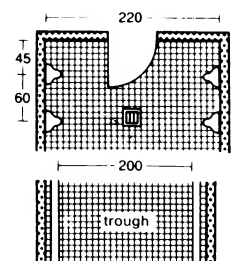
⑬ Dual row urinal bowls and troughs
